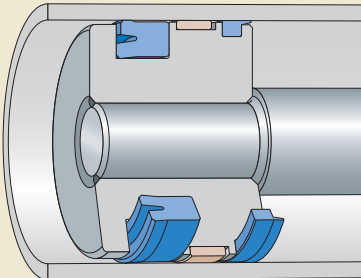
UNP profile piston seal with a wiper seal
