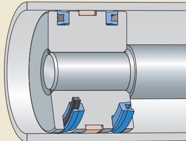
STD profiles used as piston seals (in a double-acting arrangement)
