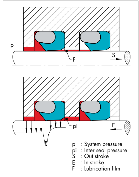
Figure 43 Pressure Distribution in Tandem Installation
