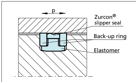
Figure 49 PHD/P Seal
