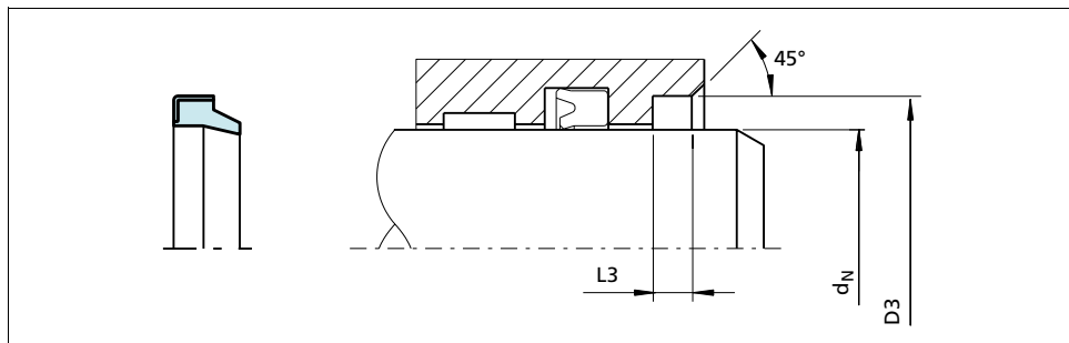
Figure 21 Installation drawing
