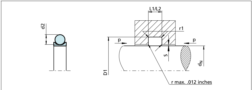
Figure 48 Installation drawing
