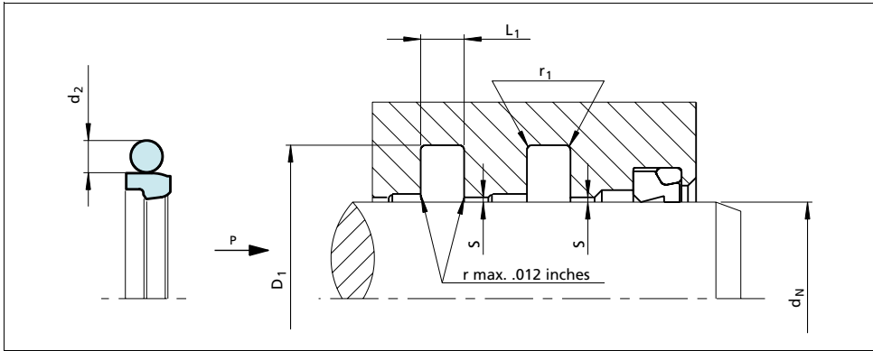
Figure 17 Installation drawing
