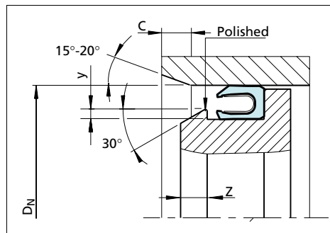
Figure 10 Installation in a half-open groove
