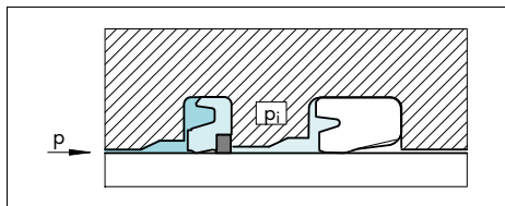
Figure 29 Tandem configuration
