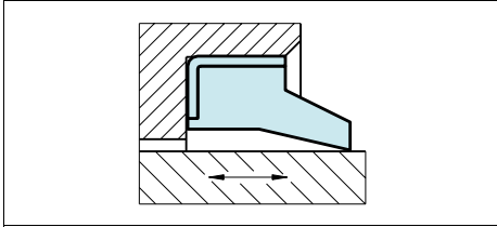
Figure 20 Scraper WSA
