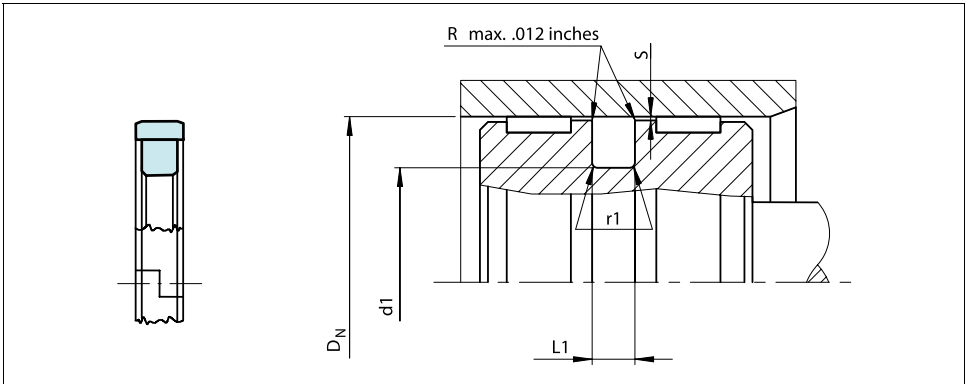
Figure 19 Installation drawing
