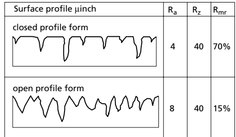
Figure 2 Profile forms of surfaces
