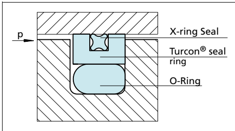
Figure 42 Turcon® AQ-Seal®
