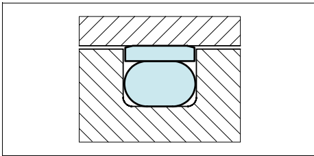
Figure 26 Turcon® Glyd Ring® C
