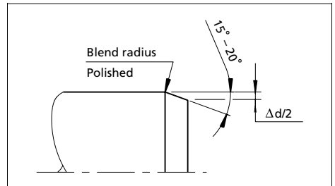
Figure 2 Lead-in chamfers
