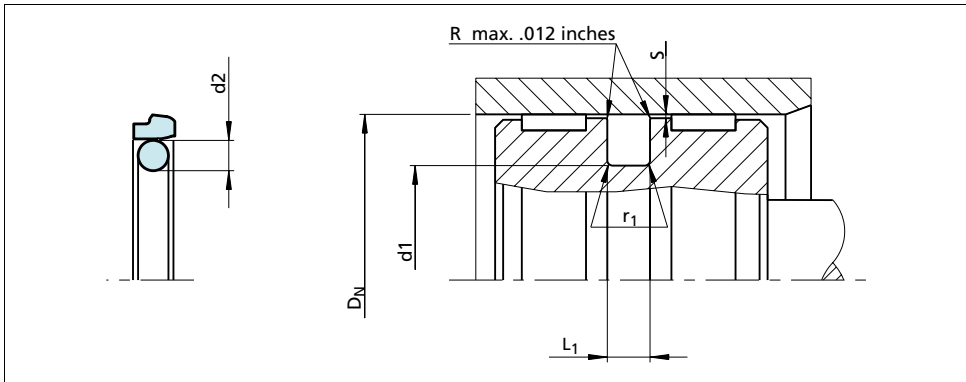
Figure 35 Installation drawing
