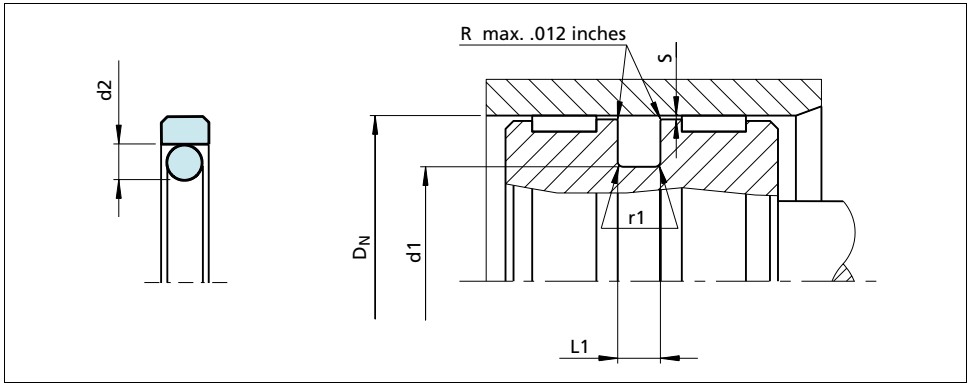
Figure 25 Installation drawing
