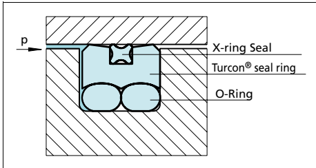
Figure 44 Turcon® AQ-Seal® 5
