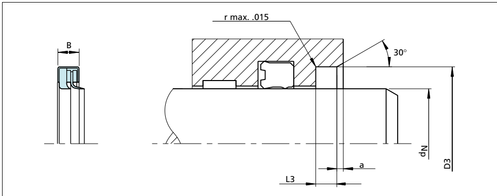
Figure 23 Installation drawing
