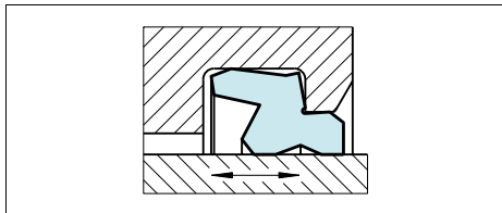
Figure 3 Scraper DA 24
