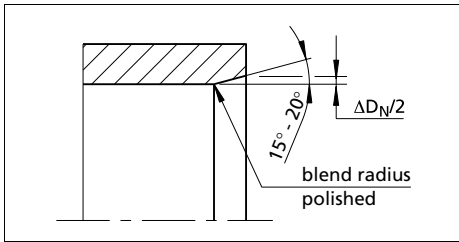
Figure 1 Lead-in chamfer
