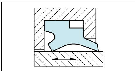
Figure 7 Scraper DA 17
