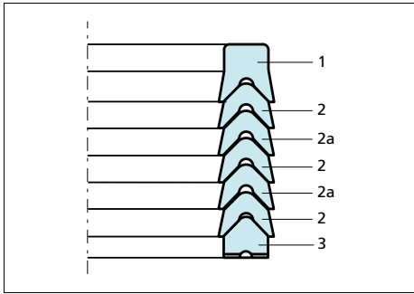
Figure 51 Veepac design
