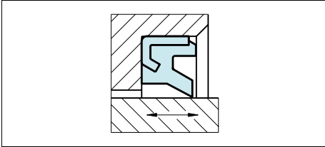
Figure 18 Scraper SWP
