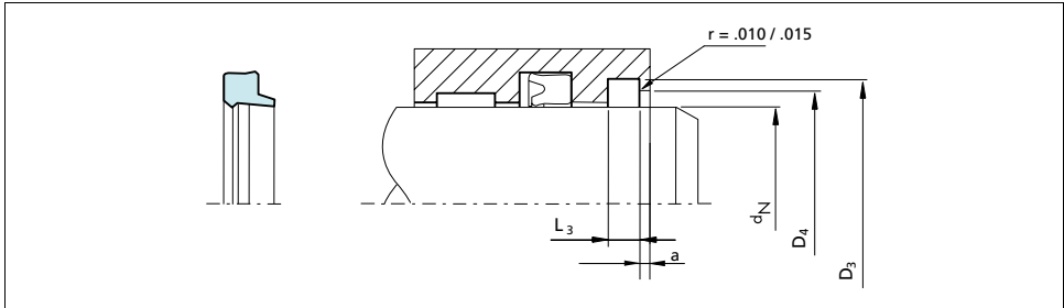
Figure 14 Installation drawing
