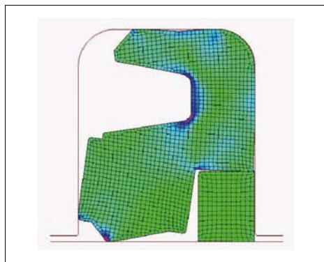
Figure 30 Zurcon® Buffer Seal un-pressurized
