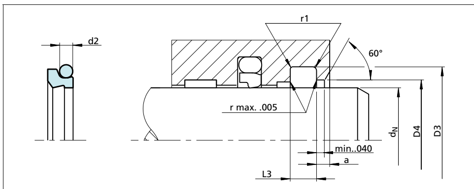
Figure 12 Installation drawing
