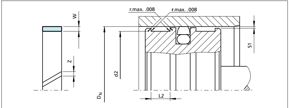
Figure 3 Installation drawing
