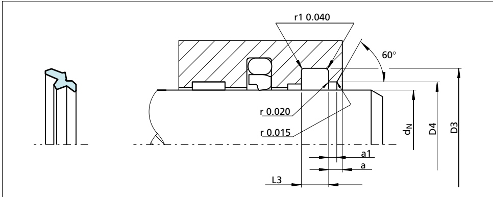
Figure 4 Installation drawing
