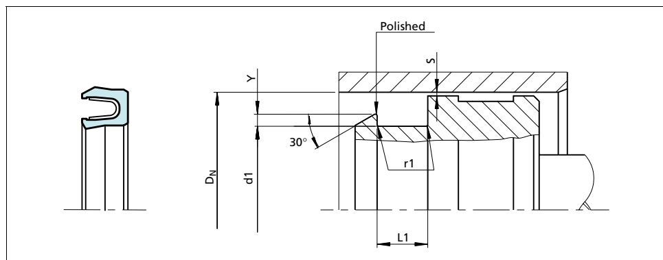
Figure 47 Installation drawing
