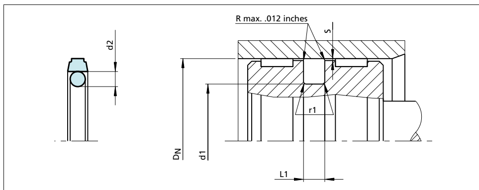
Figure 15 Installation drawing
