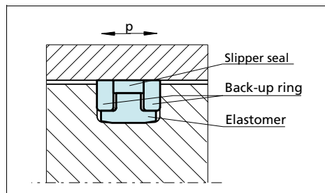
Figure 40 CST Seal
