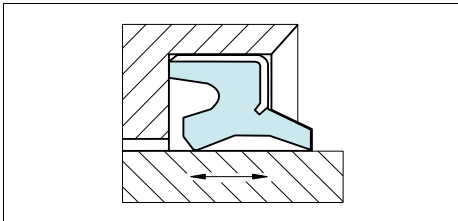
Figure 5 Scraper WKE
