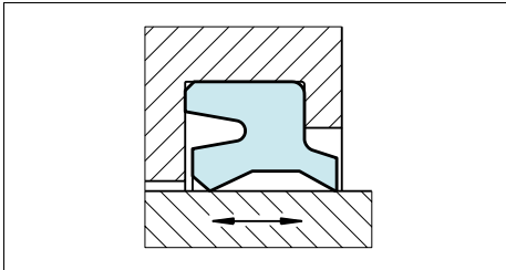
Figure 1 Scraper DA 22
