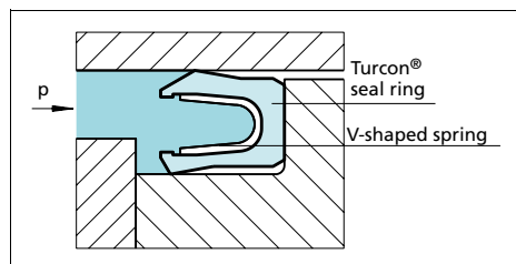
Figure 46 Turcon® Variseal® M2
