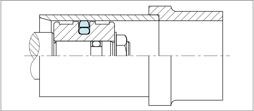
Figure 8 Sizing the sealing element with sizing sleeve
