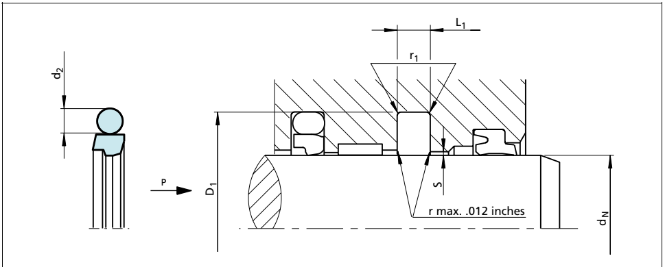
Figure 28 Installation drawing
