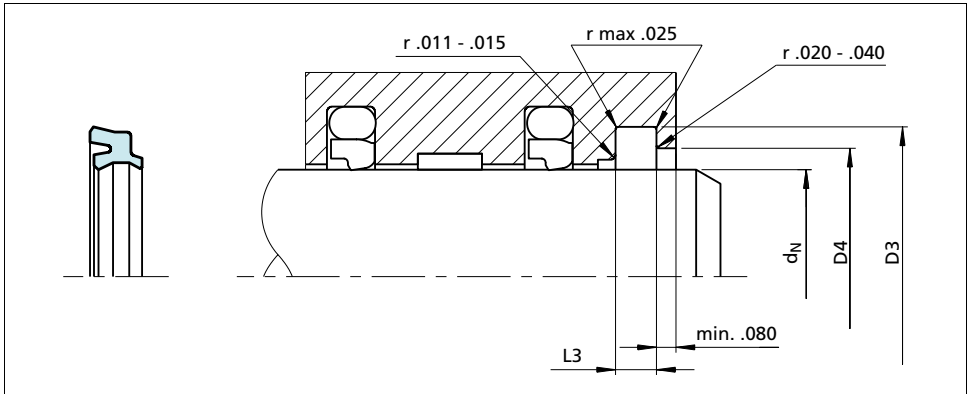
Figure 2 Installation drawing
