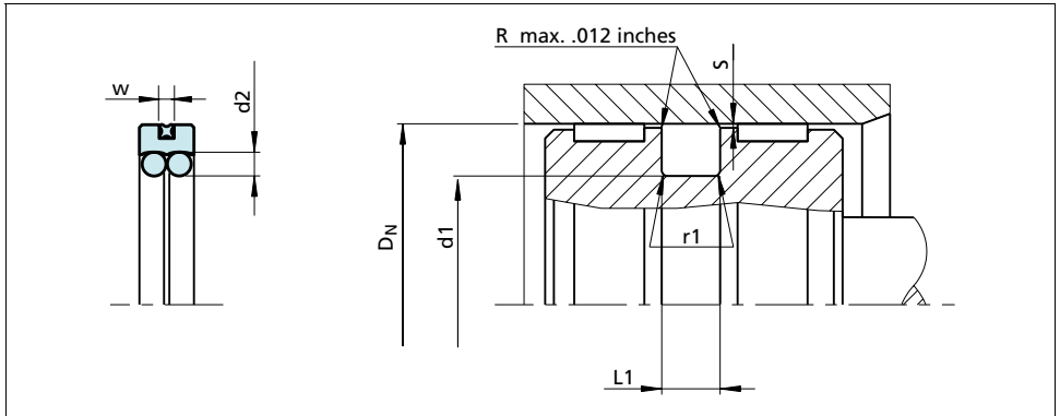
Figure 45 Installation drawing
