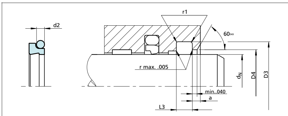
Figure 10 Installation drawing
