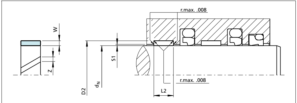
Figure 4 Installation drawing
