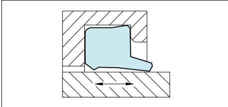
Figure 13 Scraper WAE
