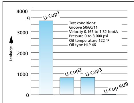
Figure 22 Leakage performance dependent on U-Cup type
